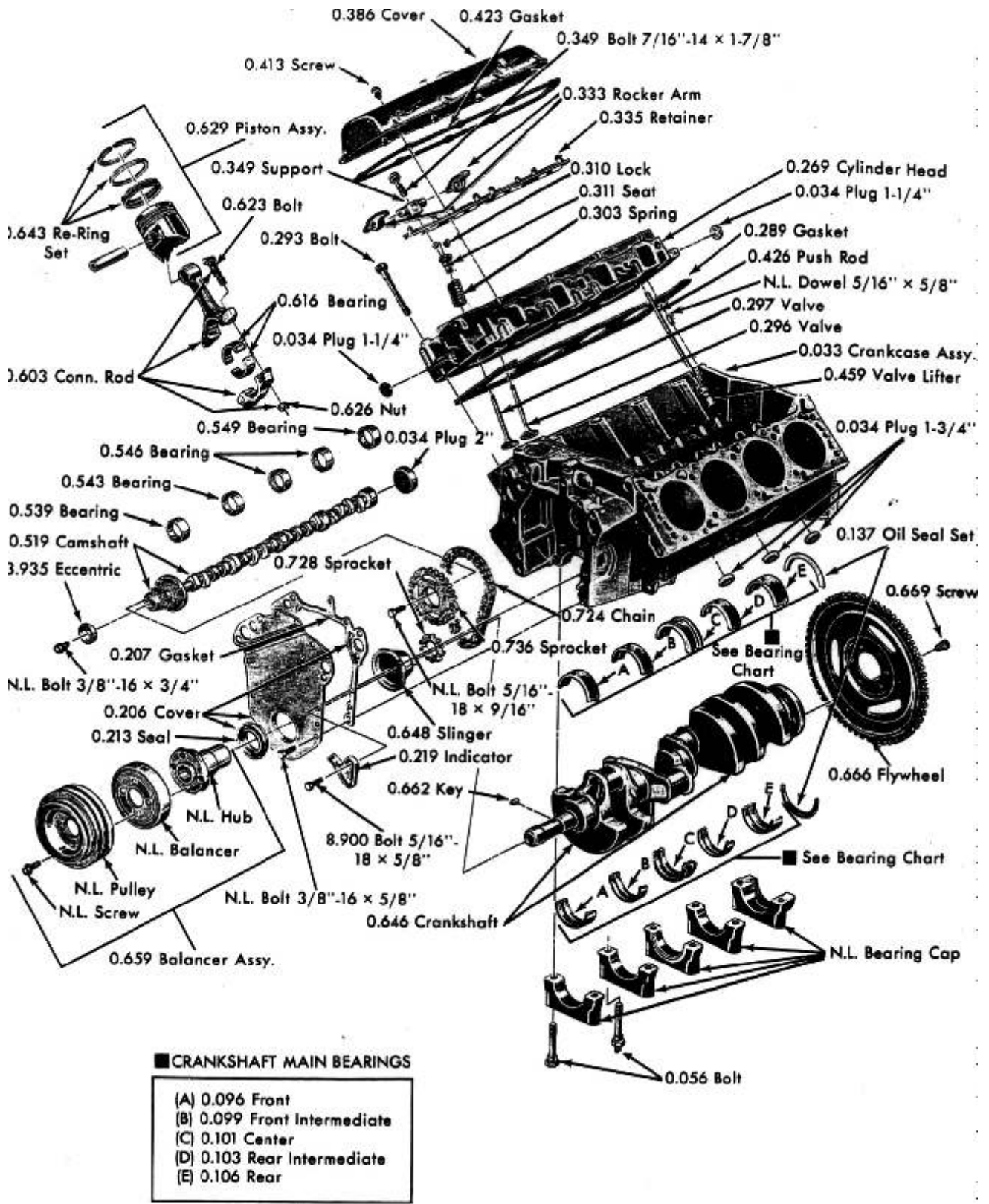
ENGINE MECHANICAL PARTS—SERIES 1968; 1969
